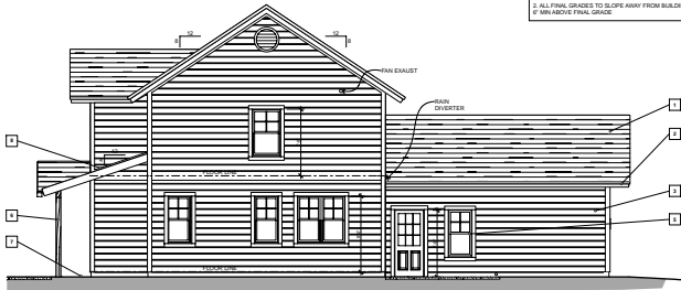
SOUTH ELEVATION 2
