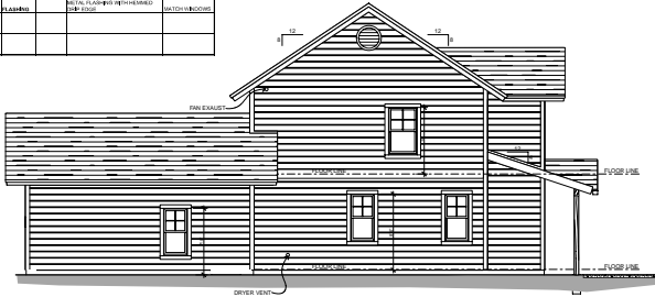
NORTH ELEVATION 1
